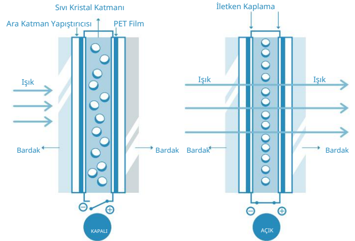
PDLC Film
